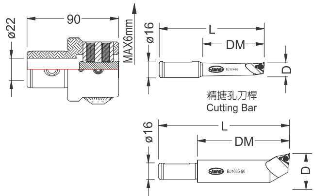
微調尺寸刻劃環 Adjust the Graduation
